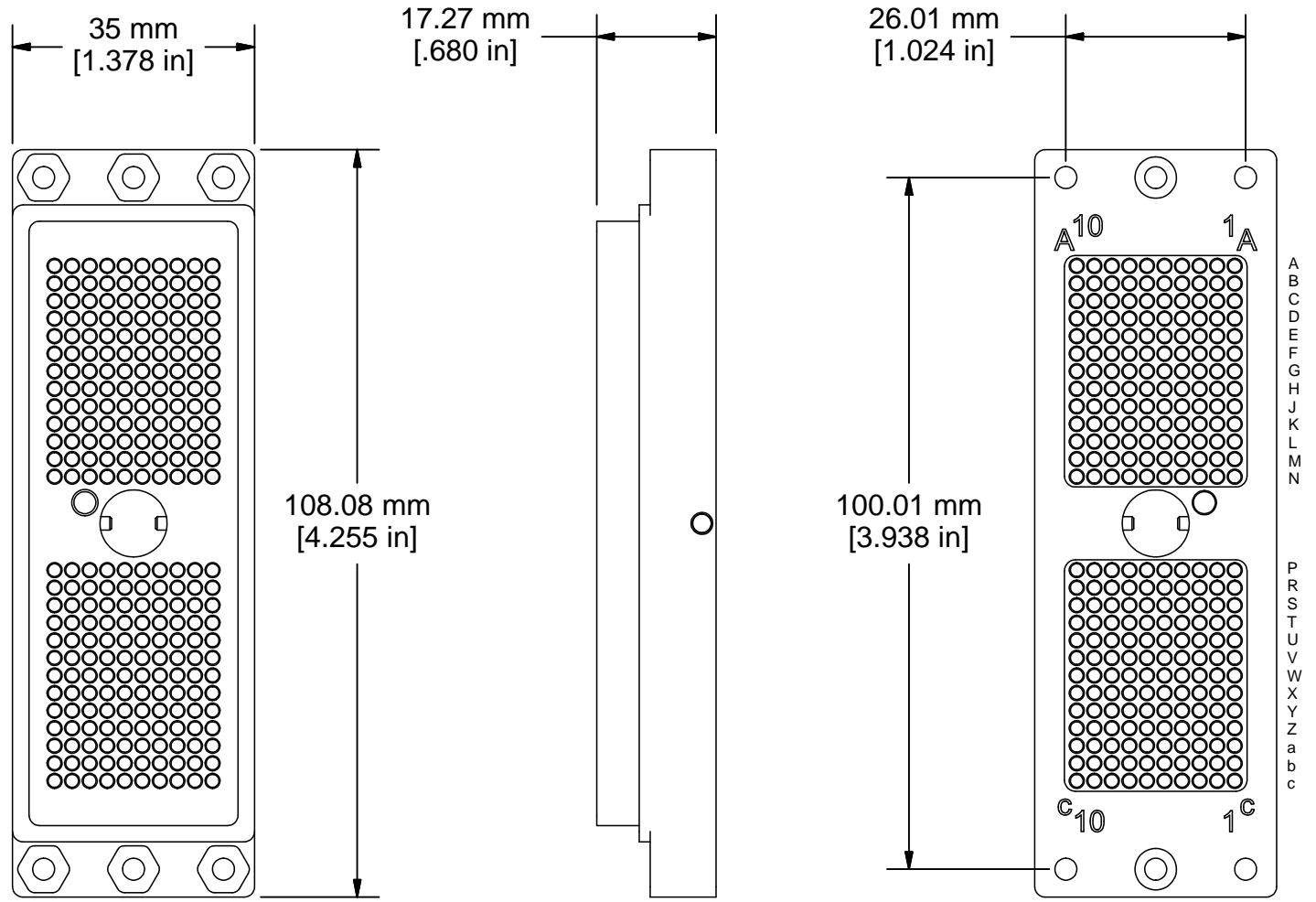
Socket Rear View
