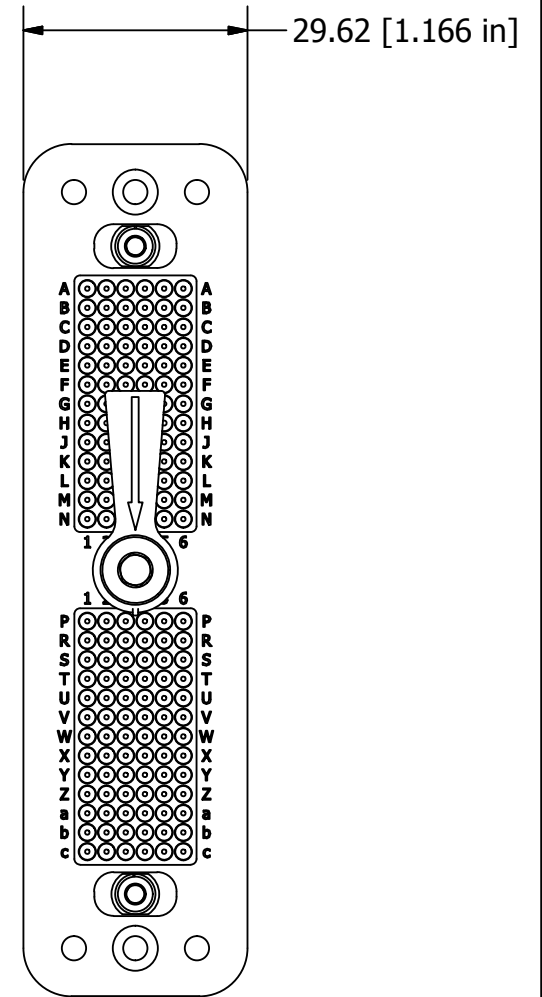
WIRING FACE VIEW
