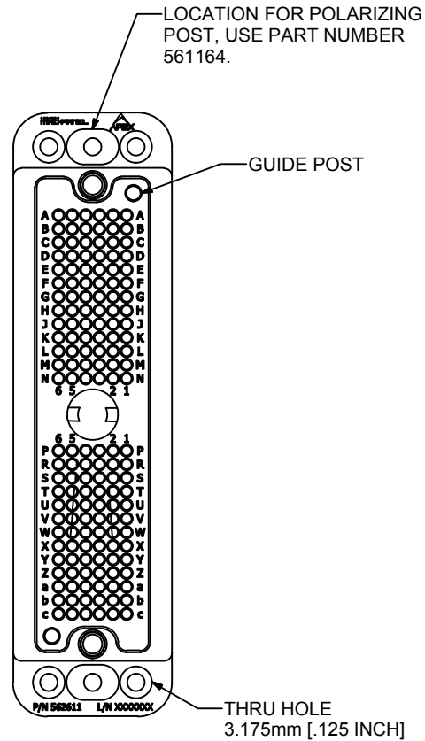
MATING FACE VIEW
