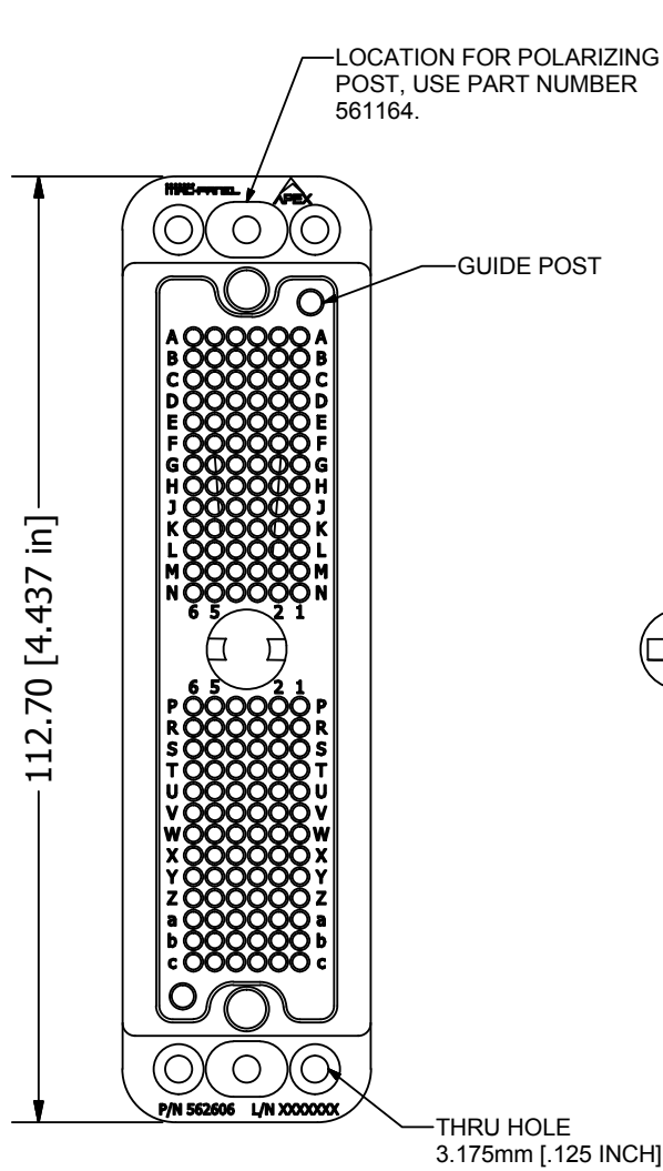
MATING FACE VIEW
