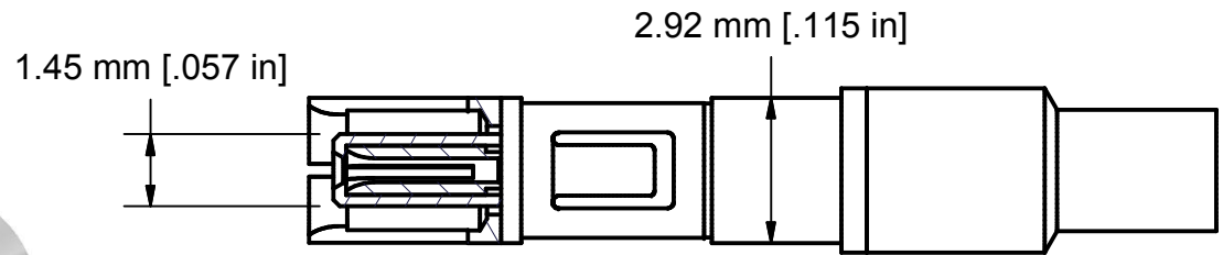
SECTION B-B
